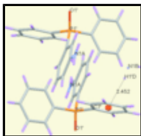
Fig. 5. N—H \cdots\pi Stacking interactions between N—H group of aniline and phenyl rings with H \cdots\pi distances of 2.45 \text{ \AA} for N1B—H1'D \cdots Cg3 ( 1 - x, 1 - y, 1 - z ) [Cg3 is the centroid for C7'–C12' ring].
