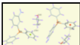
Fig. 4. C—H \cdots\pi Stacking interactions between C—H group of 2-propanol molecules with aromatic phenyl rings. The H \cdots\pi distances (measured to the center of phenyl rings) is 2.84 \text{ \AA} for C3S—H3SC \cdots Cg1 ( 1 - x, -y, 1 - z ) and 2.93 \text{ \AA} for C4S—H4SC \cdots Cg2 ( 2 - x, 1 - y, -z ) [Cg1 and Cg2 are the centroids of C13'–C18' and C7—C12 rings, respectively].
